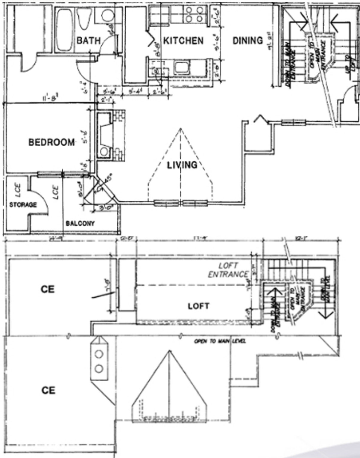
UNIT TYPE E-1A-LOFT TOTAL AREA = 1228.20 SQUARE FEET
