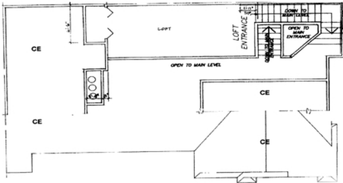
UNIT TYPE D-1A-LOFT TOTAL AREA = 1514.60 SQUARE FEET
